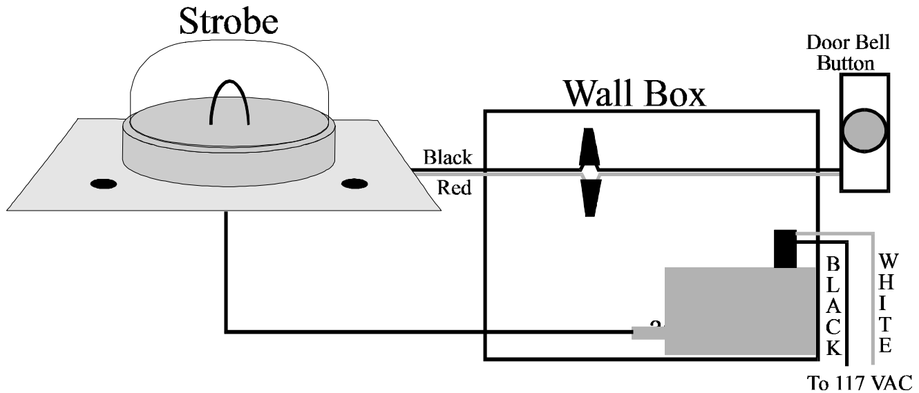
Wiring Diagram
